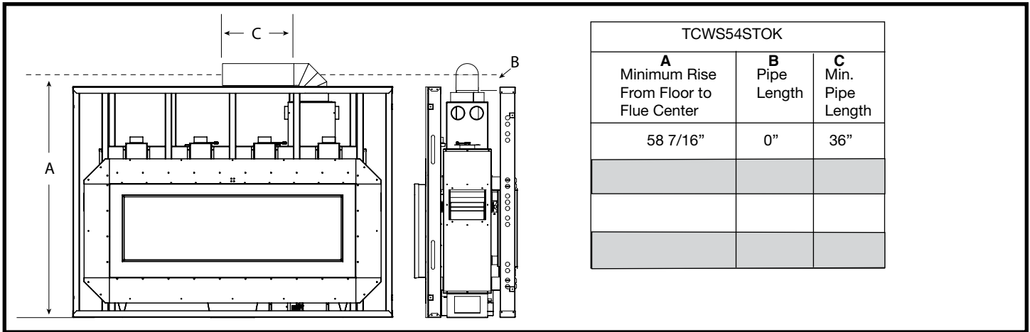
Figure 37: Minimum pipe length.
