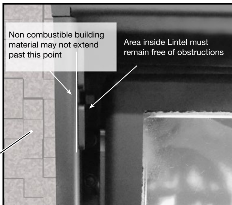
Figure 21: Framing edge location.
