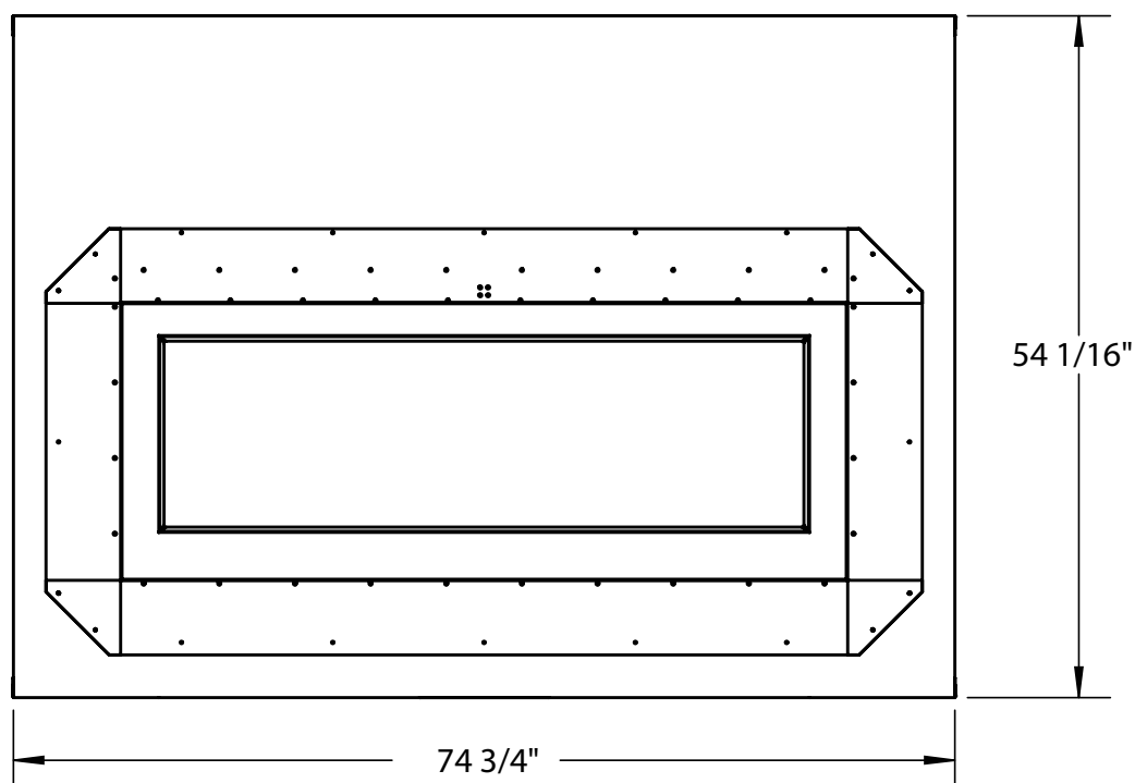
Figure 14: Outside door dimensions.
