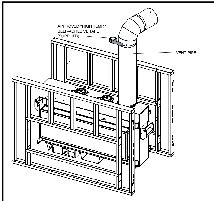
Figure 39: Taping vent pipe.
