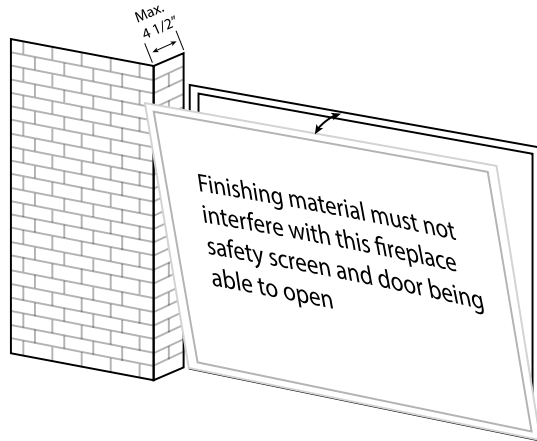
Figure 16: TCWS54STOK Recessed installation details.
