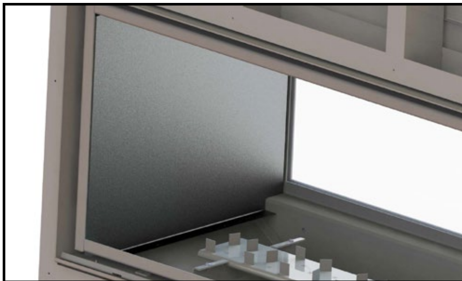
Figure 47: Side panel install.
