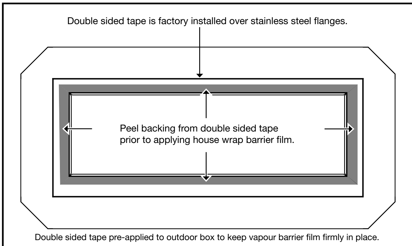
Figure 13: Double sided tape for outdoor box.
