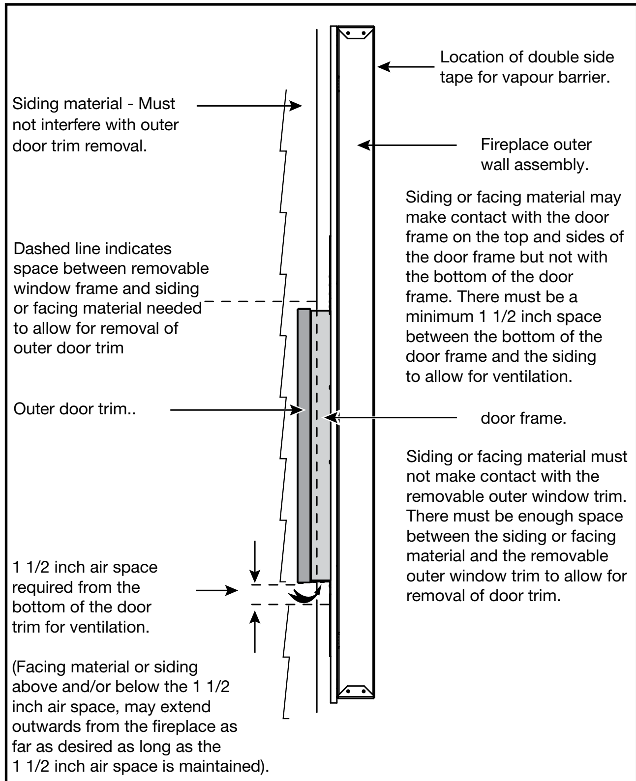
Figure 12: Outdoor-side building materials.
