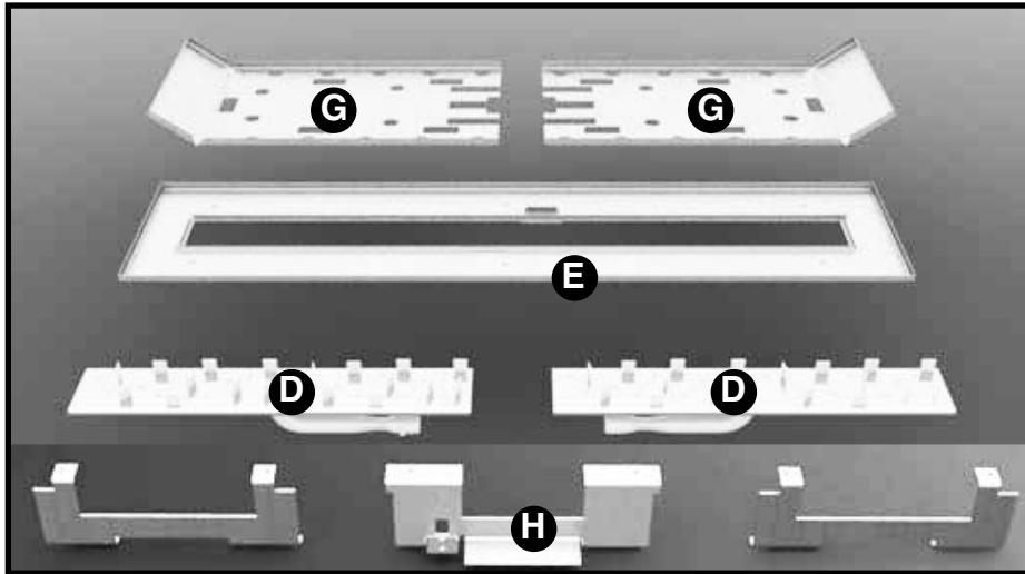
Figure 40: Tranquility kit components.
