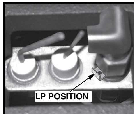
Figure 71: Pilot adjustment band in liquid propane position.
