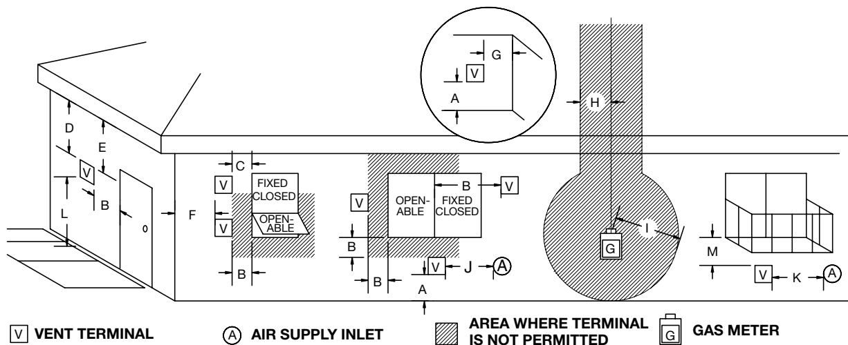
Figure 38: Vent terminal minimum clearances.
