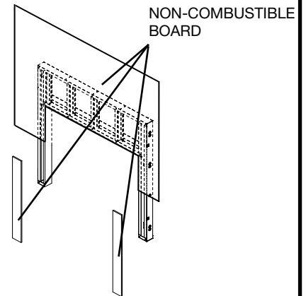
Figure 17: Non-combustible board location.
