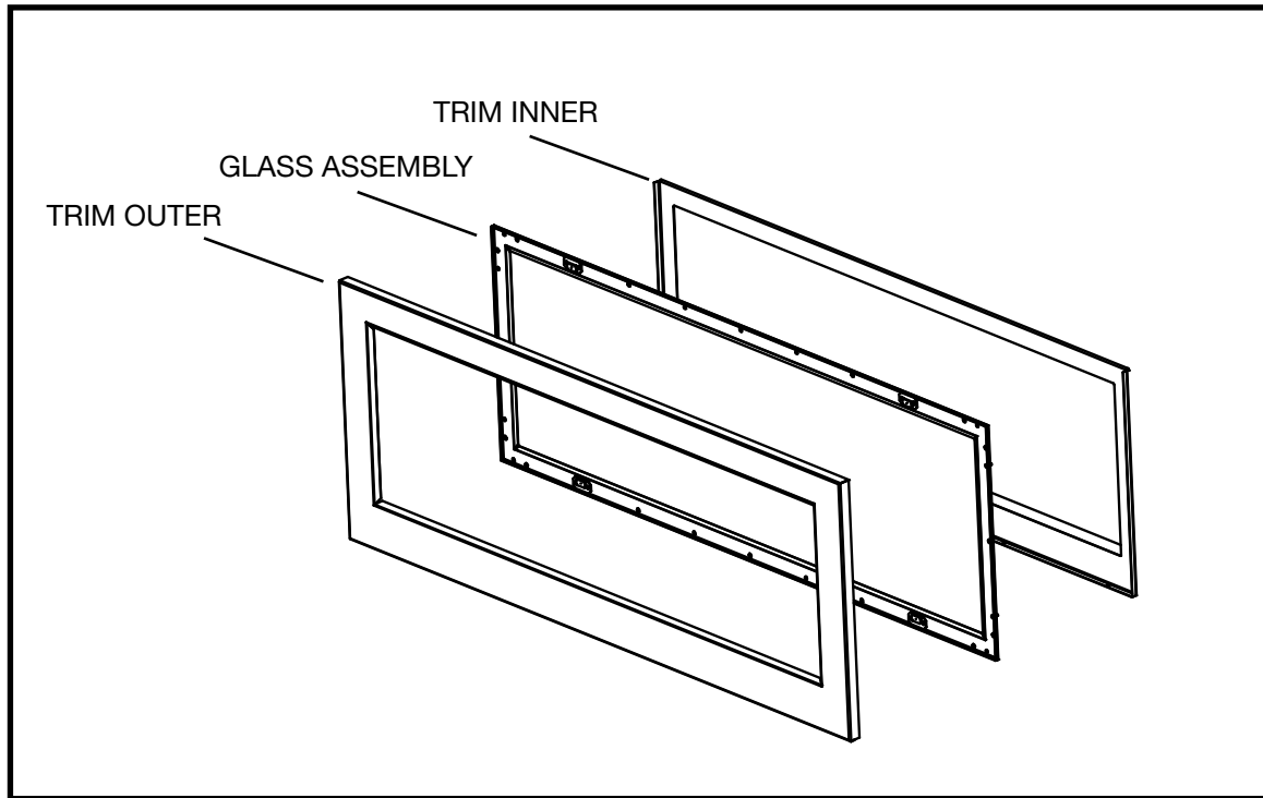
Figure 100: Door trim.
