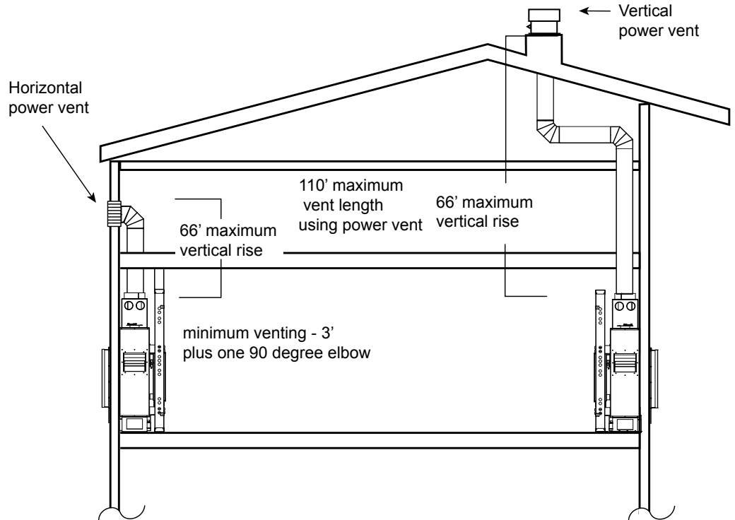
Figure 36: Venting configurations.
