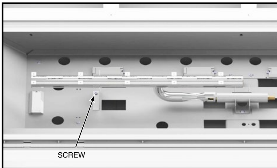
Figure 73: Installing first of two burners.
