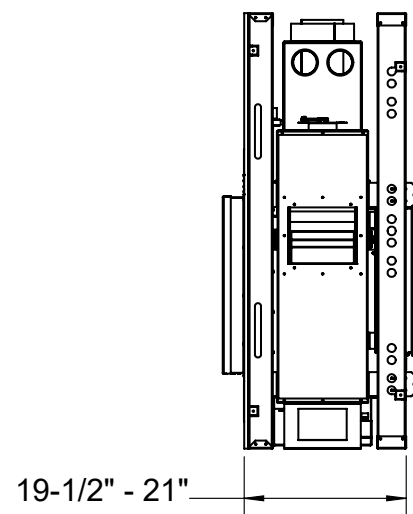
Figure 17: Non-combustible board location.
