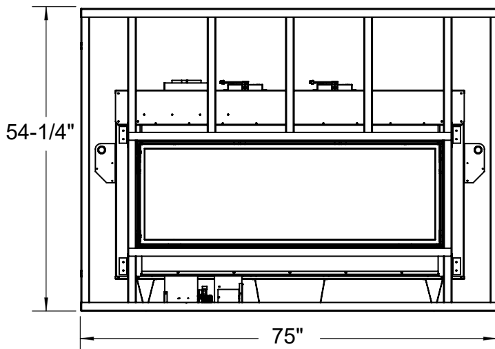
Figure 16: TCWS54STOK Recessed installation details.
