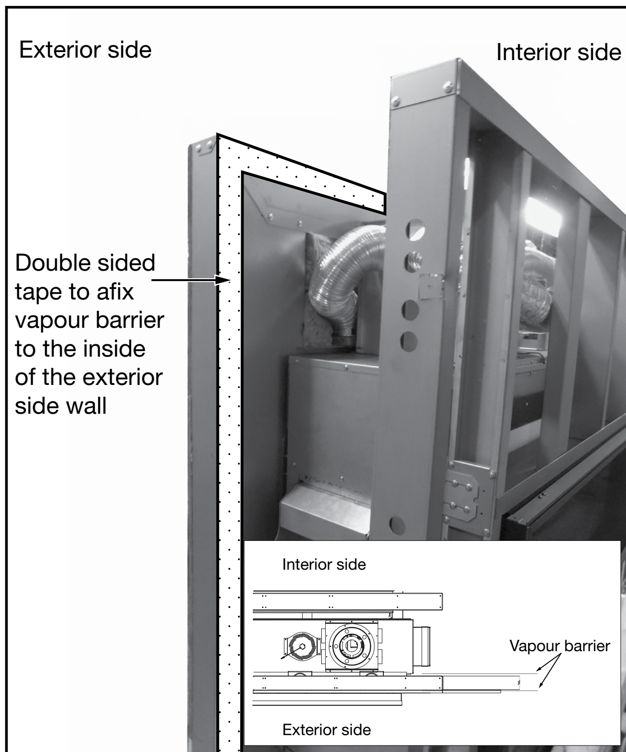
Figure 11: Tape for exterior wall vapour barrier.
