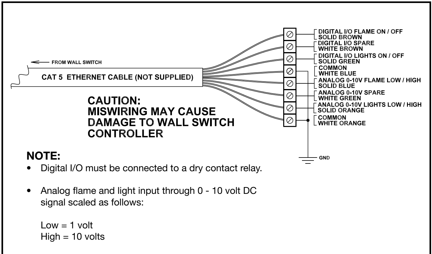
Figure 35: Home automation wiring.
