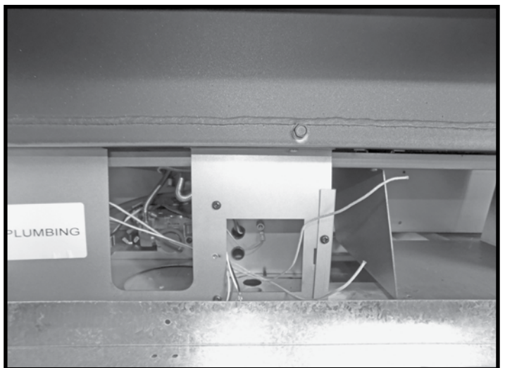
Figure 91: Bringing wires through front plate.
