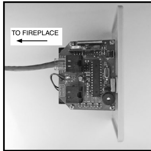
Figure 31: Wall switch - interface side.
