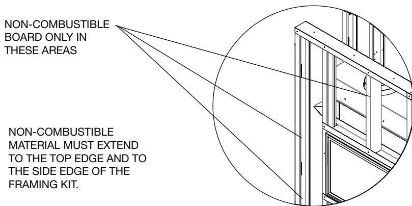
Figure 15: Non combustible board within frame.
