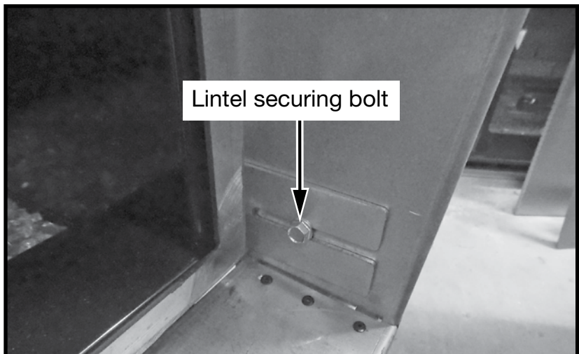
Figure 24: Lower right securing bolt.
