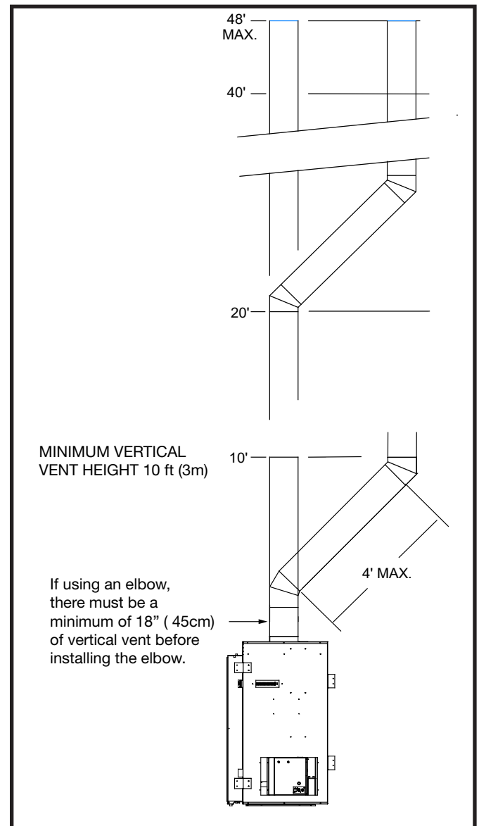
Figure 29: TCWS54CODE Venting chart.
