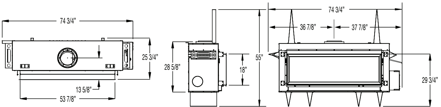
Figure 5: TCWS.54 OD with Screen dimensions.
