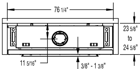
Figure 16: WS54 OD w Screen framing dimensions.
