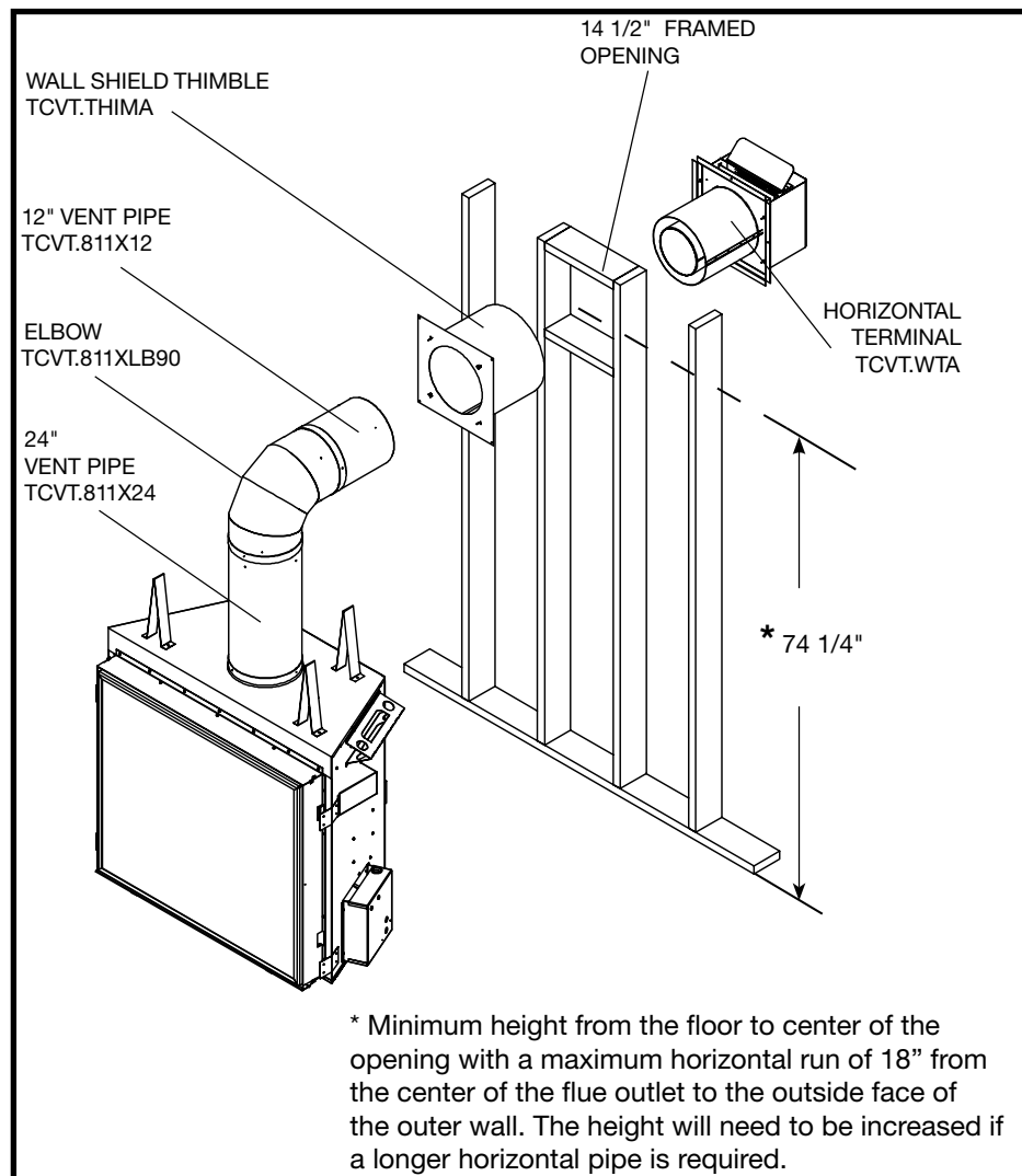
Figure 30: Wall vent terminal framing.
