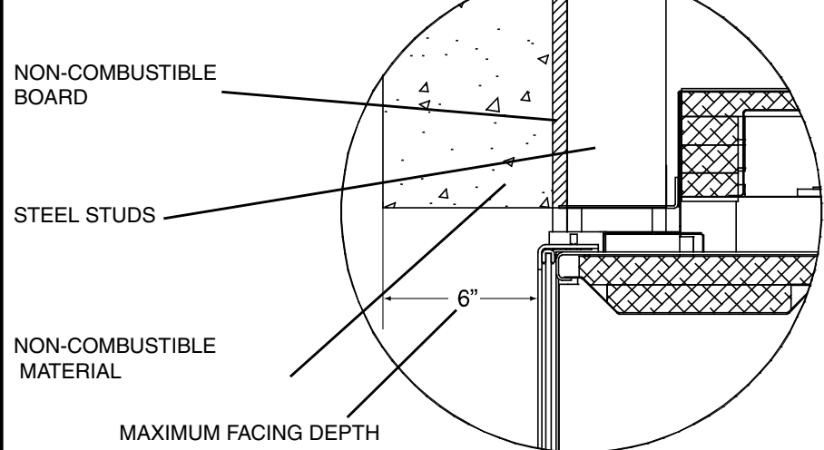
Figure 11: Non-combustible recessed installation.
