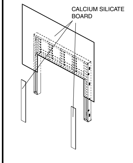
Figure 10: Calcium silicate board.
