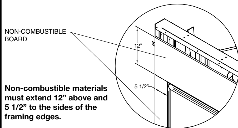
Figure 9: Non-combustible board allowances.
