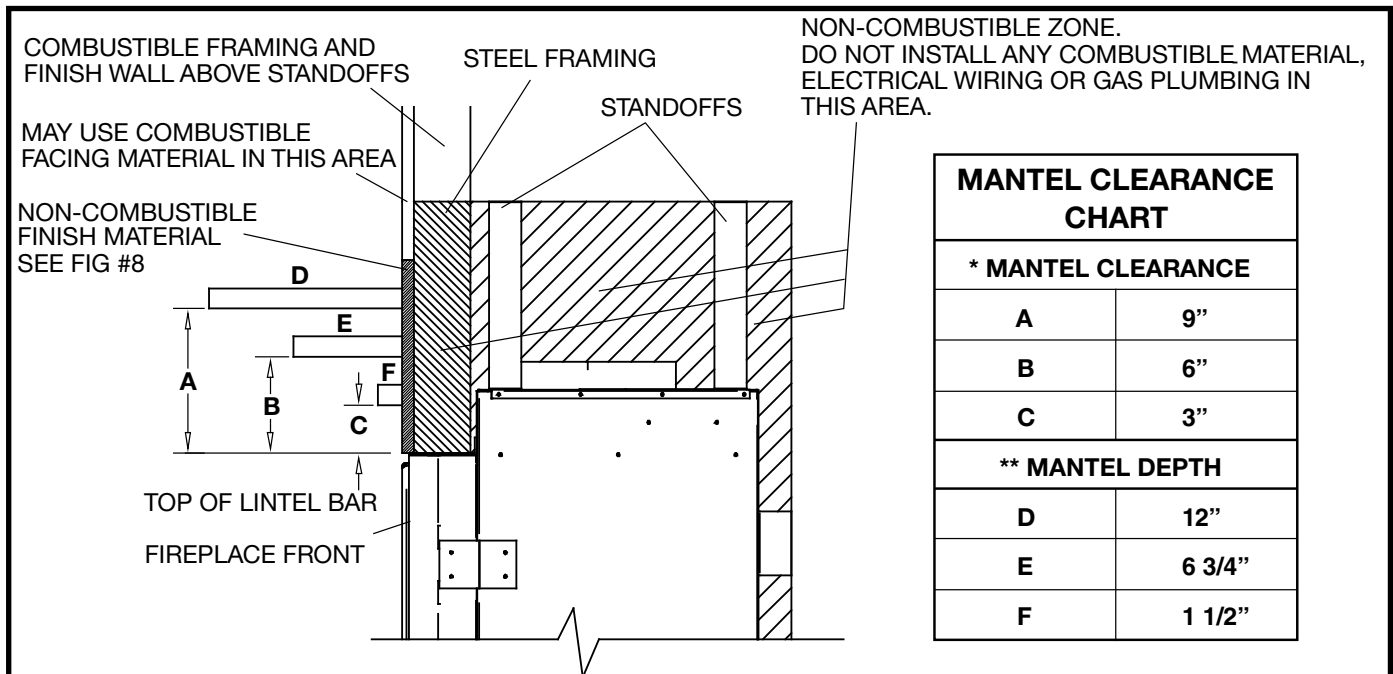
Figure 1: Mantel clearances.
