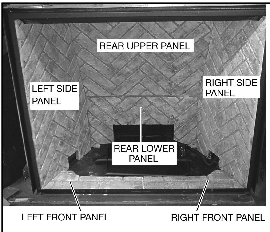
Figure 54: TC42D Panel placement.
