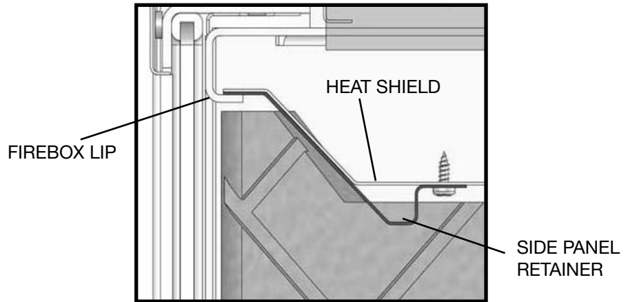
Figure 52: Side panel retainer.
