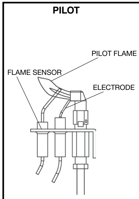
Figure 66: Pilot assembly.
