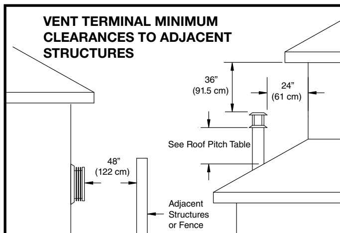
Figure 41: Vent roof clearance.
