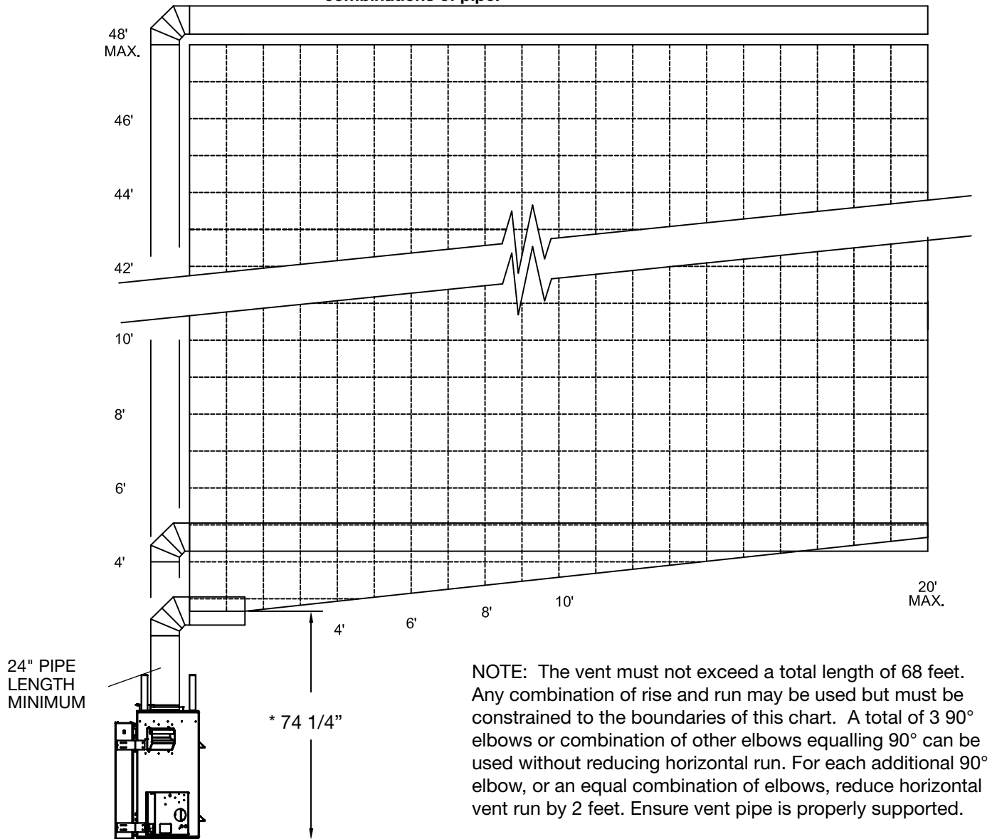
Figure 36: TC42D Horizontal run - rise chart.
